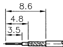
RECOMMENDED CABLE STRIPPING DIM'S (建議剝線尺寸)
