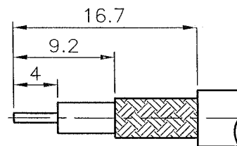
RECOMMENDED CABLE STRIPPING DIM'S (建議剝線尺寸)
