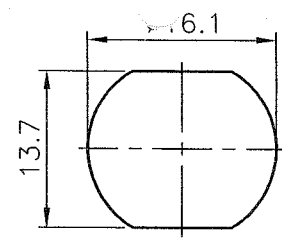
RECOMMENDED MOUNTING HOLE (建議架設孔)
