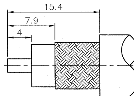
RECOMMENDED CABLE STRIPPING DIM'S (建議剝線尺寸)
